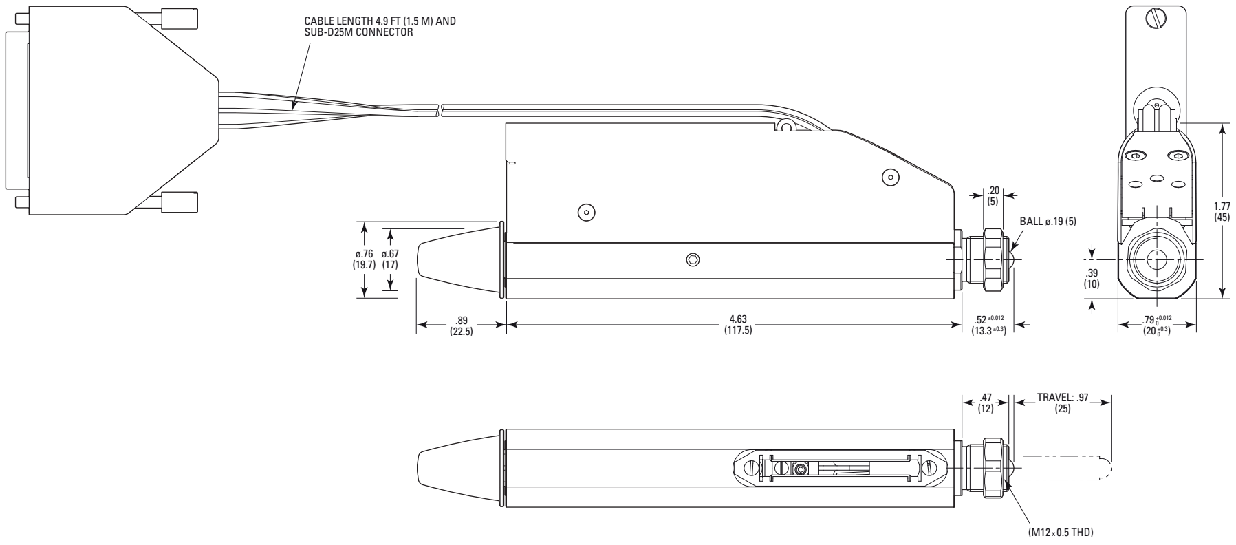
MODEL SHOWN: LTAHLPPV6 DIMENSIONS IN INCHES (AND MILLIMETERS) 0 5 10 20 30 IN. (MM) SCALE 3:4
